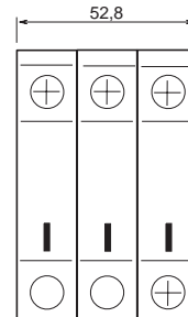
3 poles
