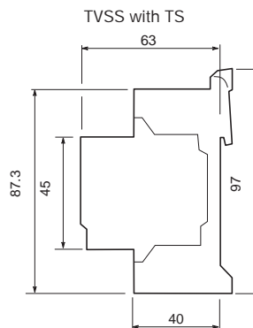
3 poles
