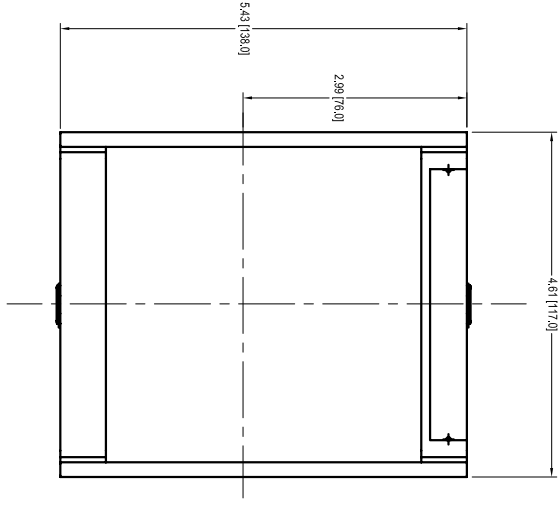
FLANGE FOR COMPARTMENT DOOR
