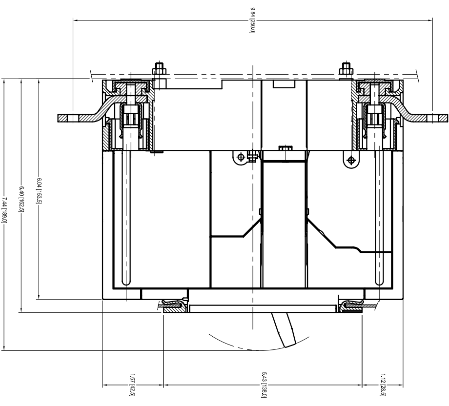
SIDE VIEW
