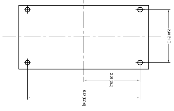
DRILLING TEMPLATES FOR SUPPORT SHEET
