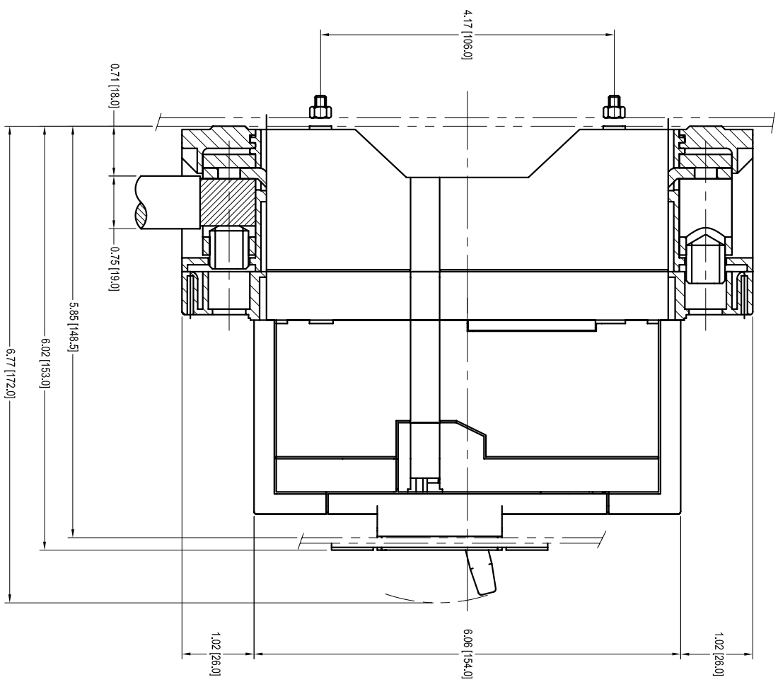
SIDE VIEW
