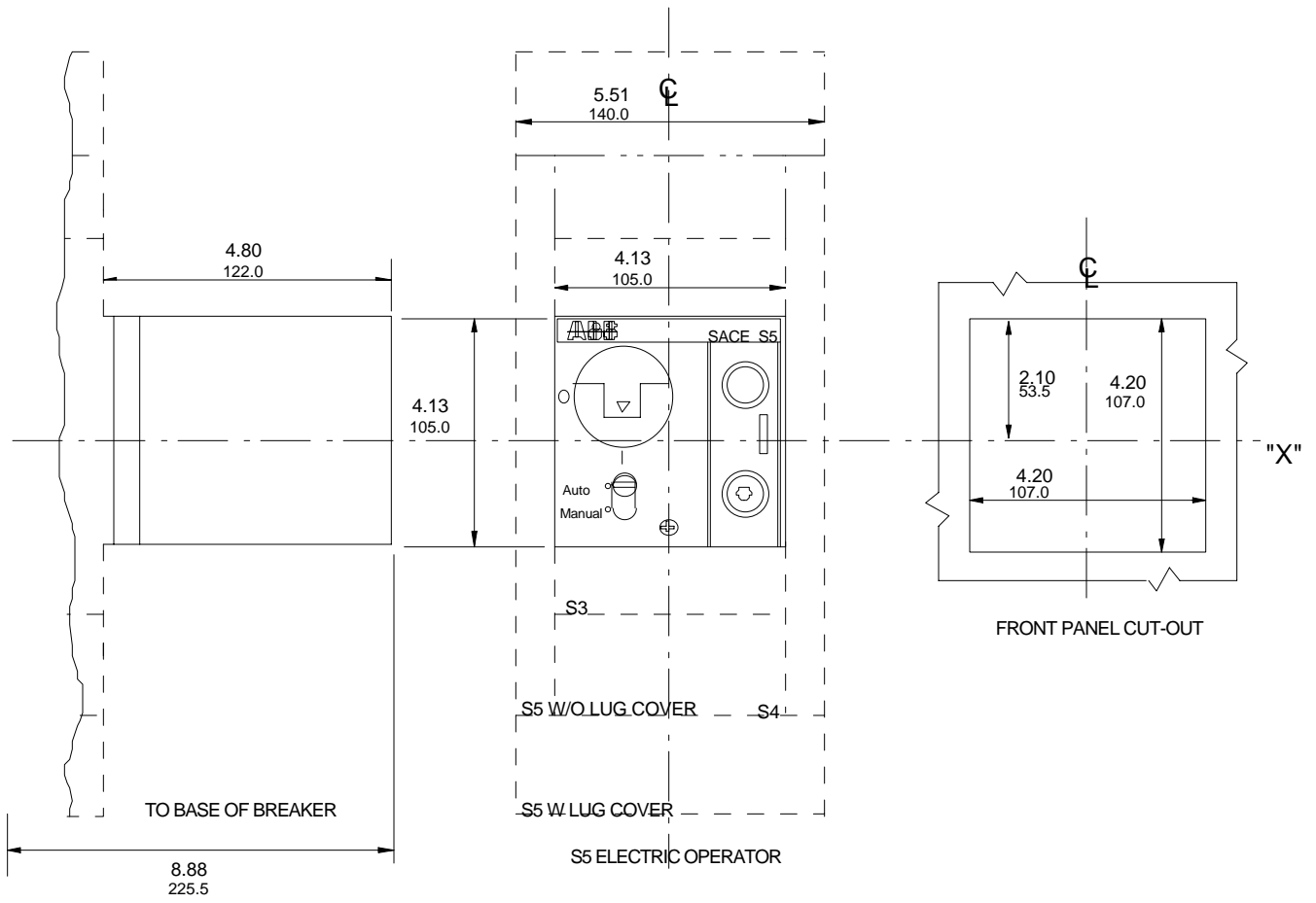
S5 ELECTRIC OPERATED
