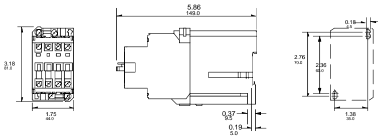
ABB Control Inc. 1-23-96 KC RELAY / 8 POLE
