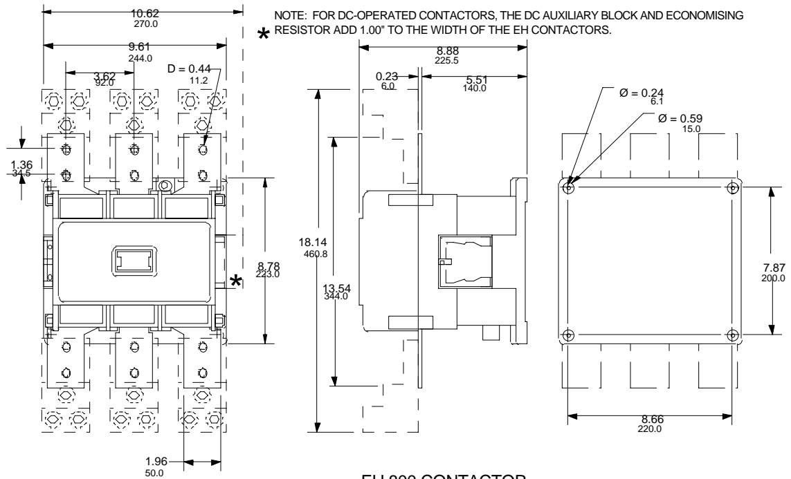
EH 800 CONTACTOR
