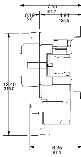
EH175Reversing Starter W/EHTK210
