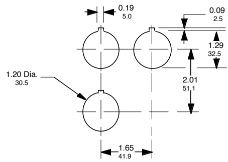
CBG DRILL PLANS
