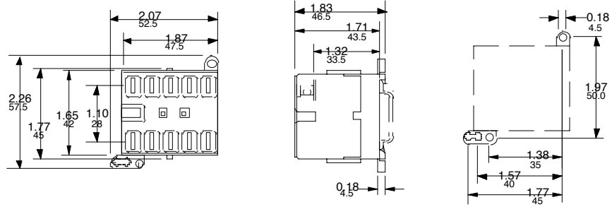
B6, BC6, K6, & KC6 WITH FLAT PINS CONNECTION
